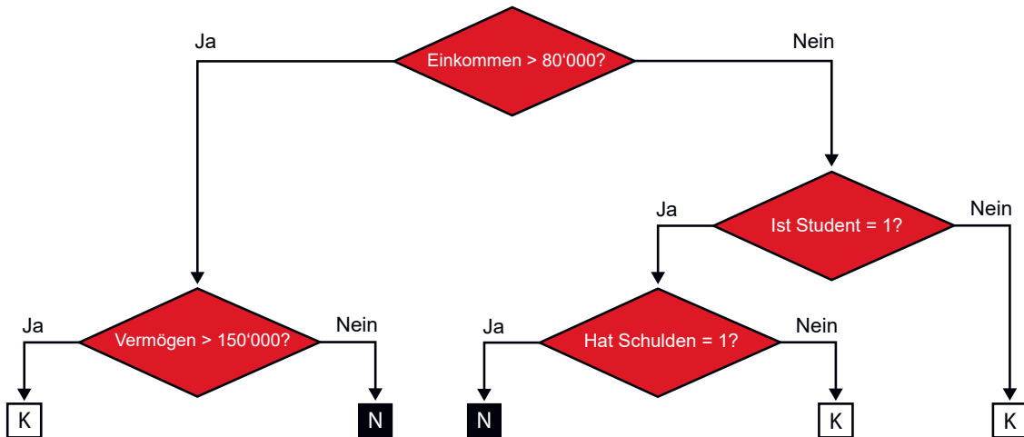
Abbildung 16: Decision Tree
