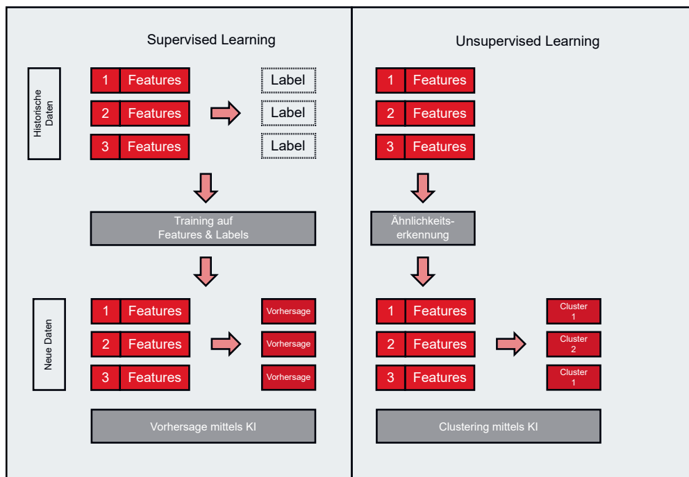
Abbildung 14: Differenz Supervised Learning/Unsupervised Learning
